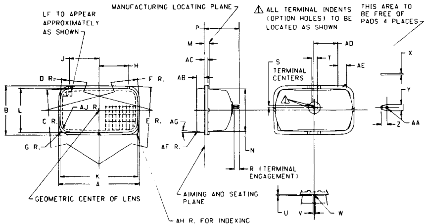
FIG. 11 - TYPE LF RECTANGULAR SEALED BEAM HEADLAMP UNIT
