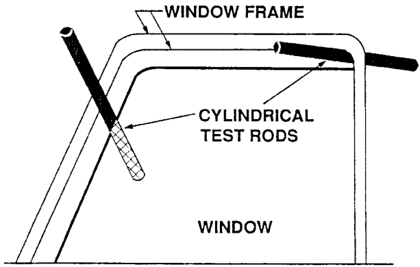
Figure 1 - Typical Cylindrical Test Rods Protruding through Sunroof and Window Daylight Openings
