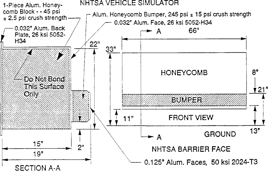
NHTSA SIDE IMPACTOR - MOVING DEFORMABLE BARRIER FIGURE 2
