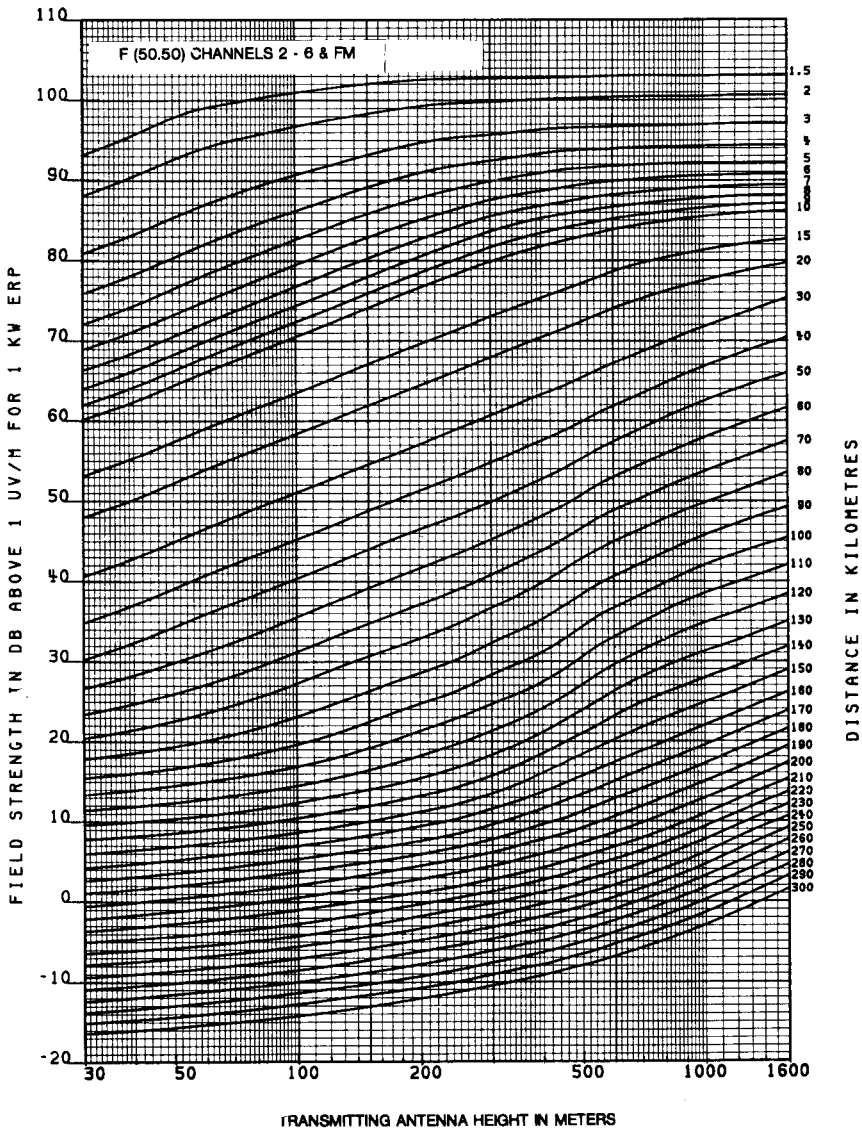
FCC 73.699 Figure 9
