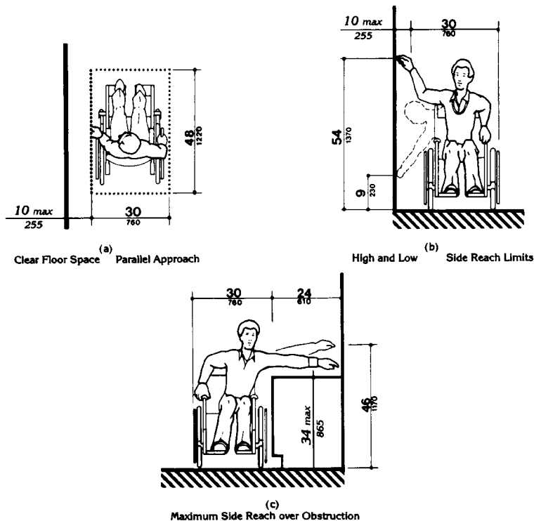
Fig. 6 Side Reach
