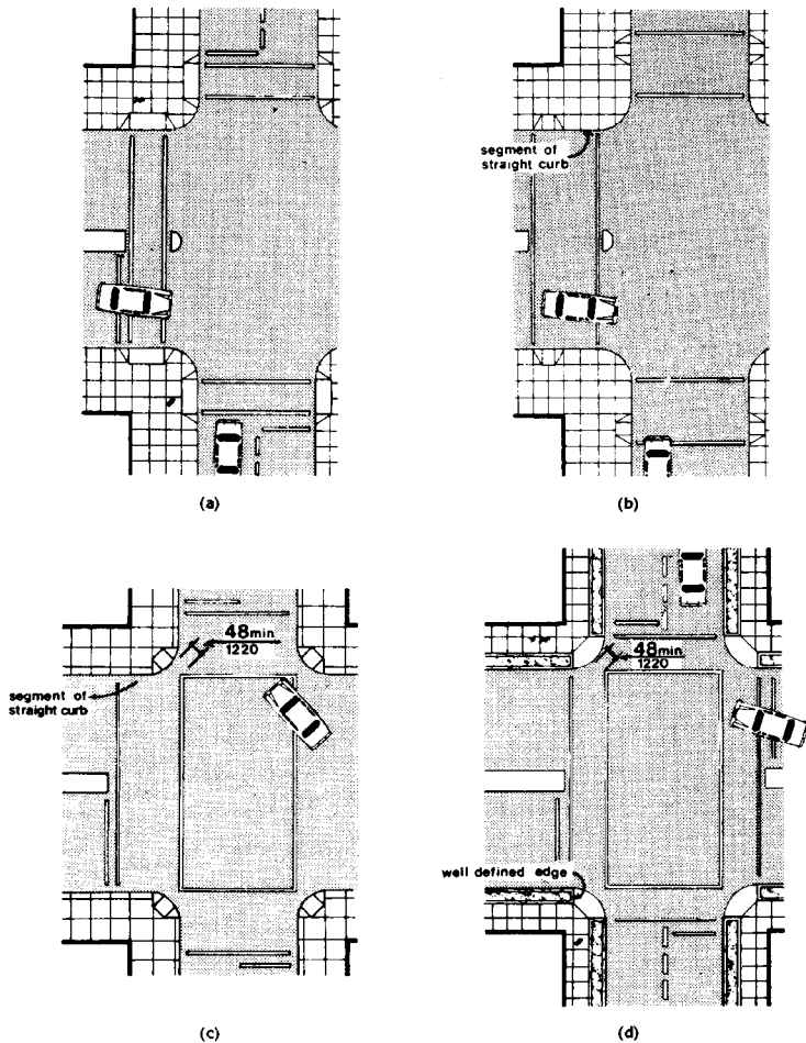
Fig. 15 Curb Ramps at Marked Crossings
