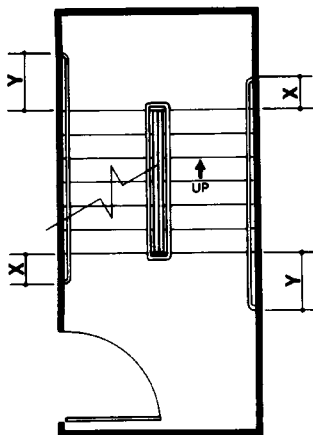
(a) Plan
