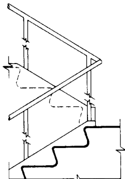
(b) Elevation of Center Handrail
