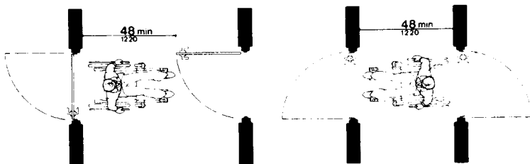
Fig. 26 Two Hinged Doors in Series
