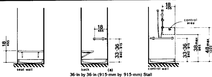
36-in by 36-in (915-mm by 915-mm) Stall
