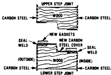
JOINT DETAIL DOT SPECIFICATION 21PF-1A OVERPACK
