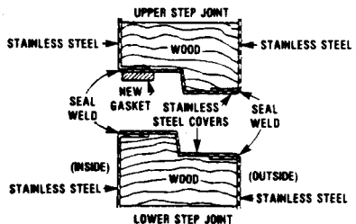
JOINT DETAIL DOT SPECIFICATION 21PF-1B OVERPACK
