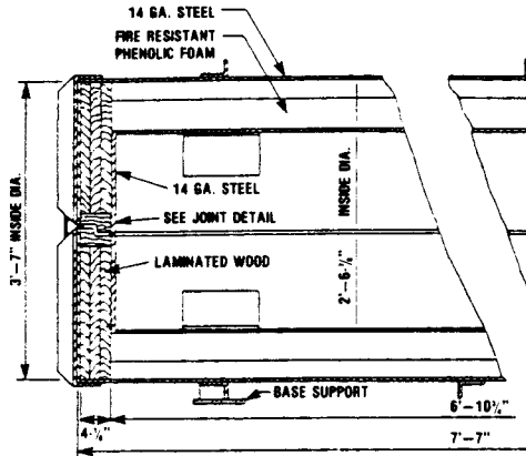
SECTION DOT SPECIFICATION 21PF-1A OVERPACK
