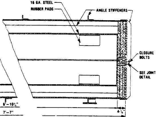
SECTION DOT SPECIFICATION 21PF-1B OVERPACK
