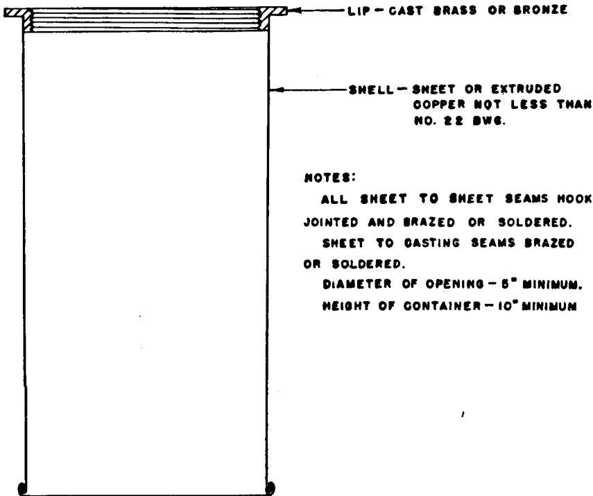
SECTIONAL VIEW
