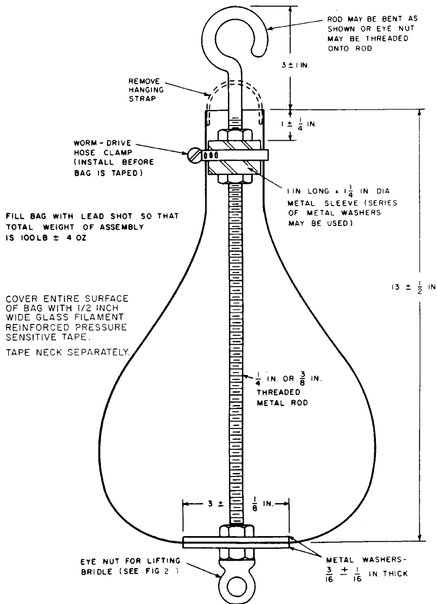
FIG 5 - IMPACTOR
