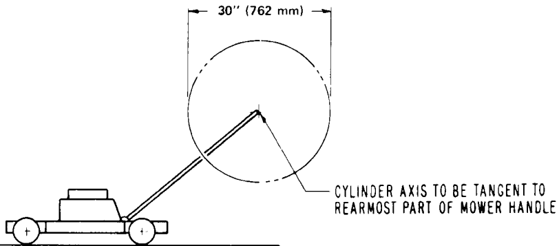
FIGURE 1 – OPERATING CONTROL ZONE
