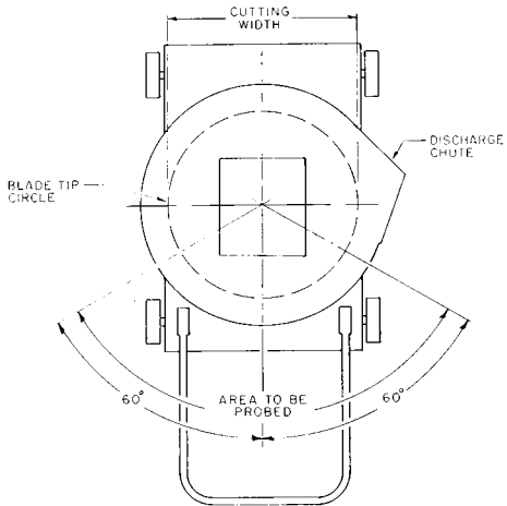
FIGURE 3 - AREA TO BE PROBED
