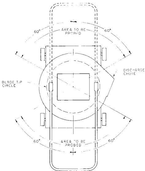
FIGURE 5 - AREA TO BE PROBED SWINGOVER HANDLE
