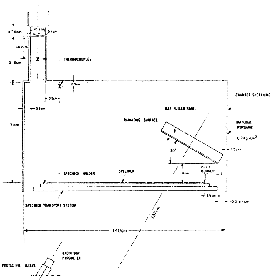
FIG 3 — FLOORING RADIANT TESTER SCHEMATIC
