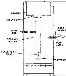
LEFT VIEW
