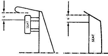
FIGURE 12. STABILITY TEST LOCATION OF CENTER OF GRAVITY OF WEIGHTS: STARBOARD SIDE
