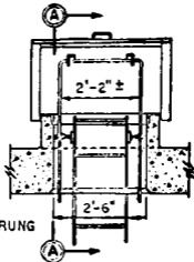
SECTIONAL ELEVATION
