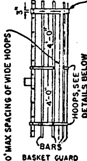
TOP AND BOTTOM HOOPS ALSO THIS SIZE
