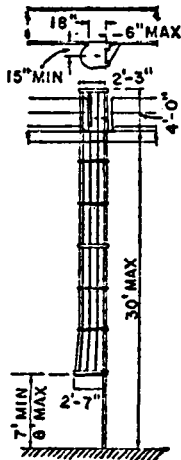
ACCESS Laterally FROM LADDER
