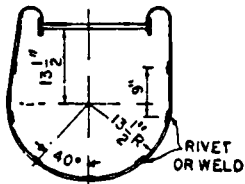
BASKET GUARD HOOP
