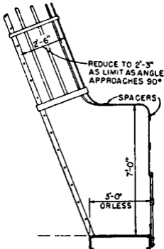
INCLINED LADDER AT ELEVATED LOCATION (FOR SPECIAL HAZARD ONLY)
