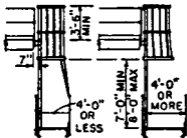
SHORT LADDERS AT ELEVATED LOCATIONS
