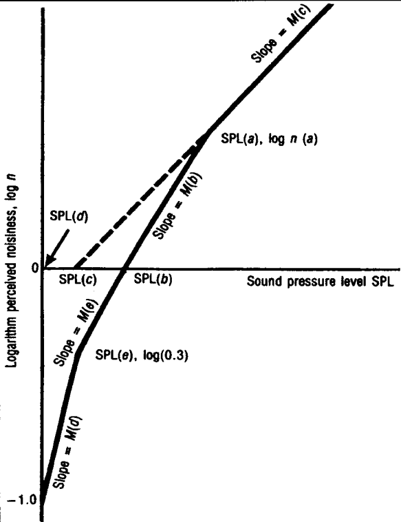
Figure A36-3. Perceived noisiness as a function of sound pressure level
