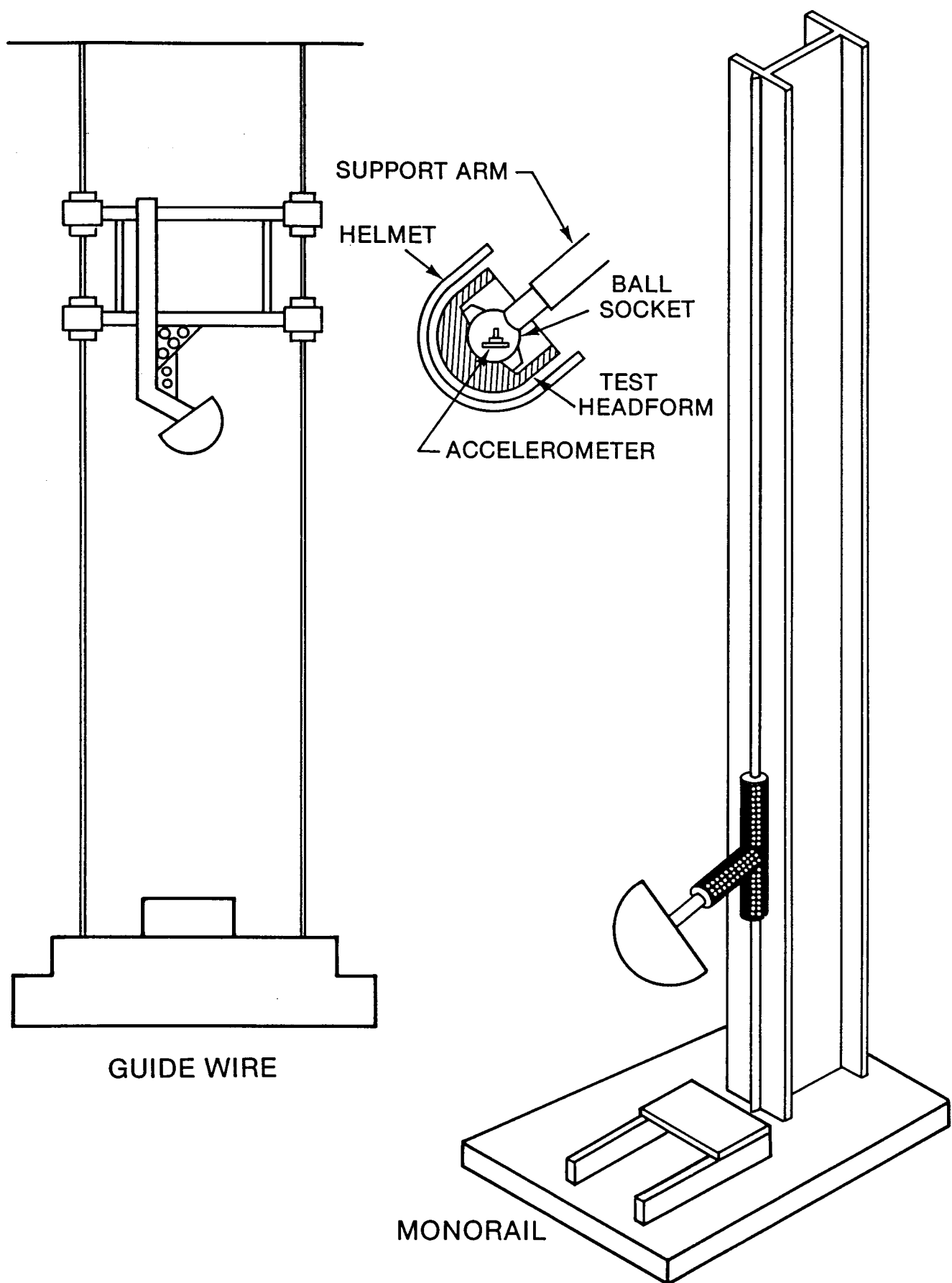
Figure 9. Impact Test Apparatus
