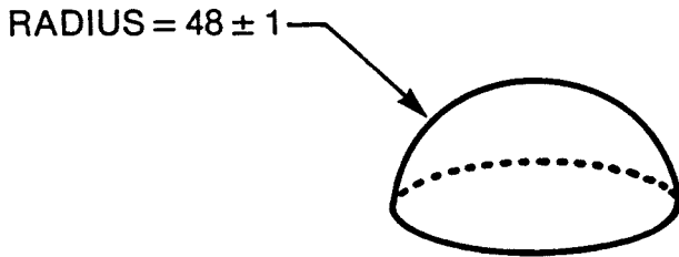
Figure 12. Hemispherical Anvil
