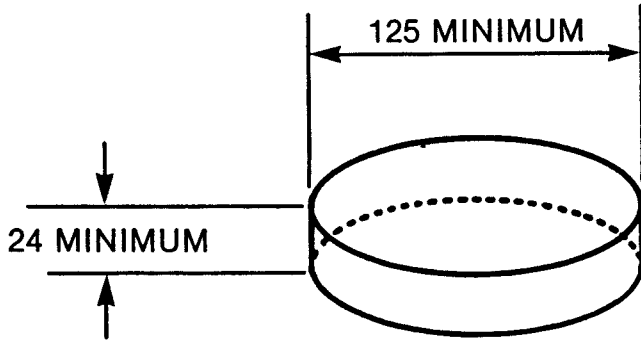
Figure 11. Flat Anvil
