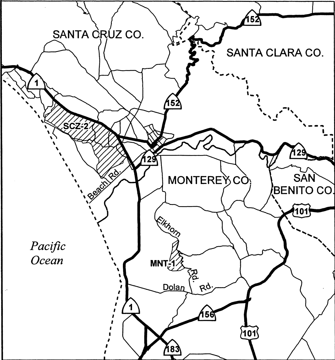
Map 13. California Red-Legged Frog Final Critical Habitat Units SCZ-2 and MNT-1
