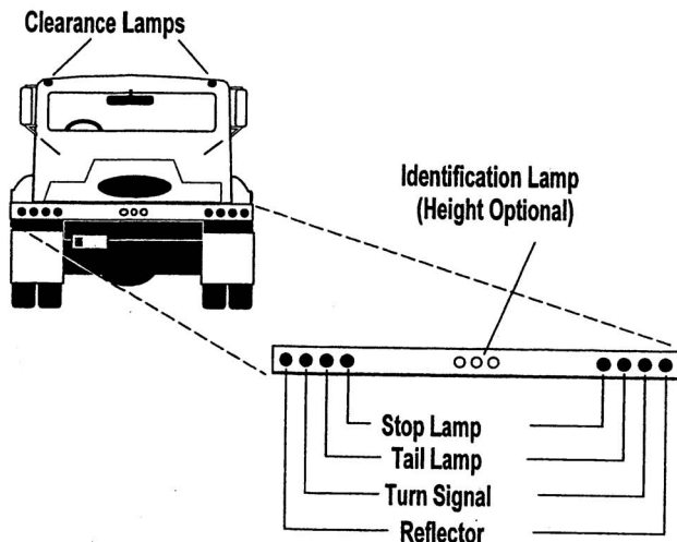
Rear of Towed Vehicle
