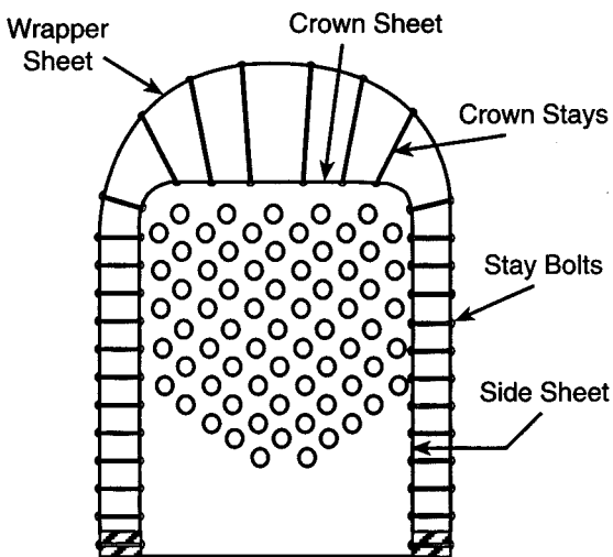
SECTION THROUGH FIREBOX
