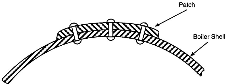
Typical Riveted Patch Installation
