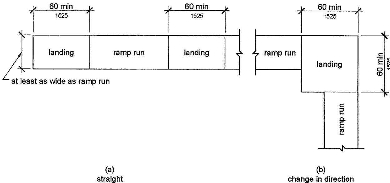
Figure 405.7 Ramp Landings
