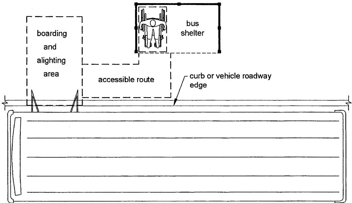
Figure 810.3 Bus Shelters
