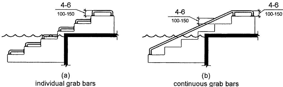
Figure 1009.5.7 Grab Bars
