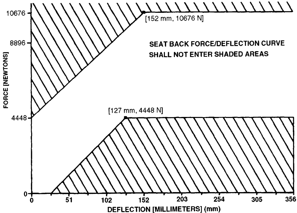
Figure 1.—Force/Deflection Zone
