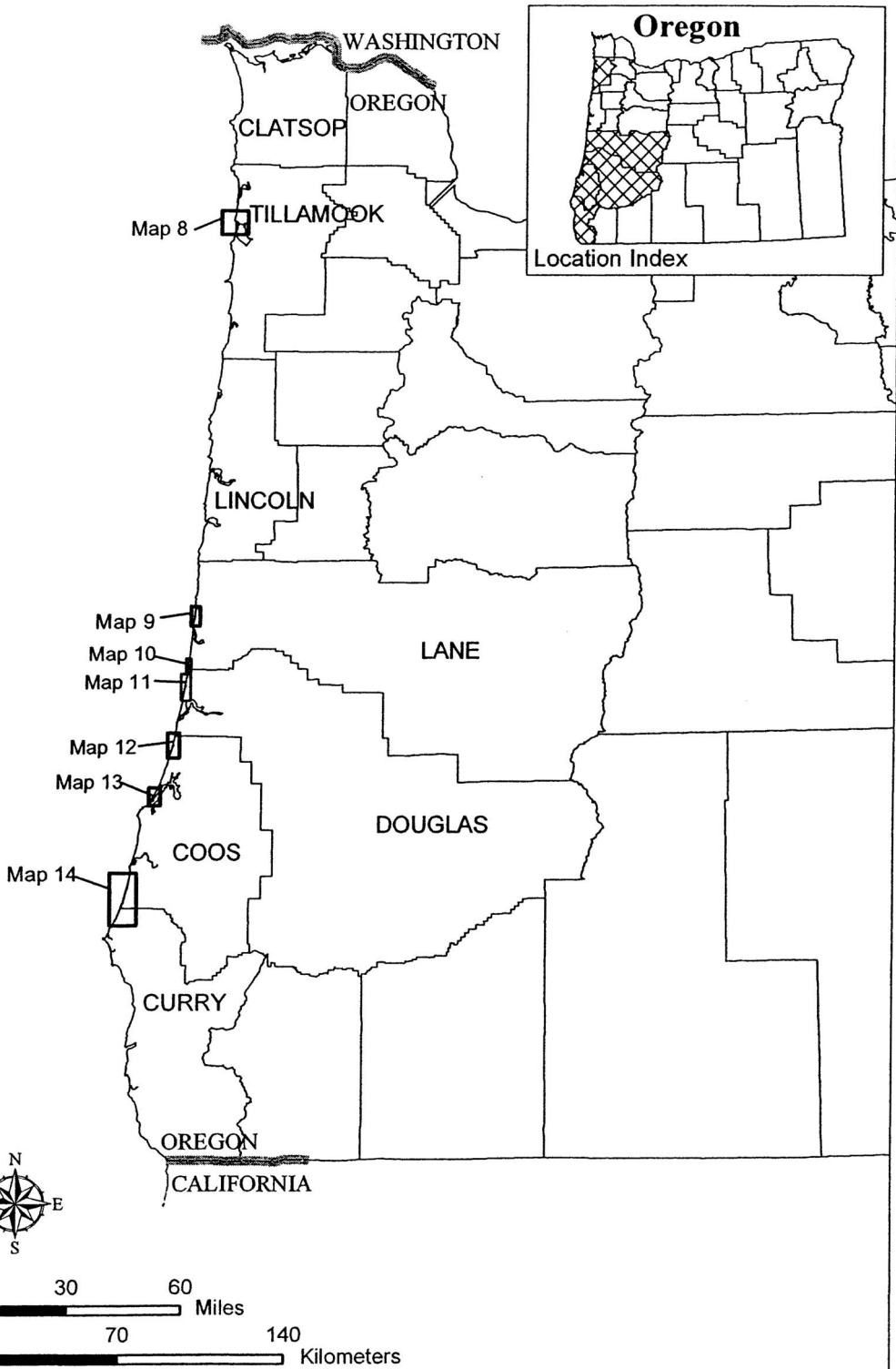
Figure M-2. Western Snowy Plover Proposed Critical Habitat, Oregon.
