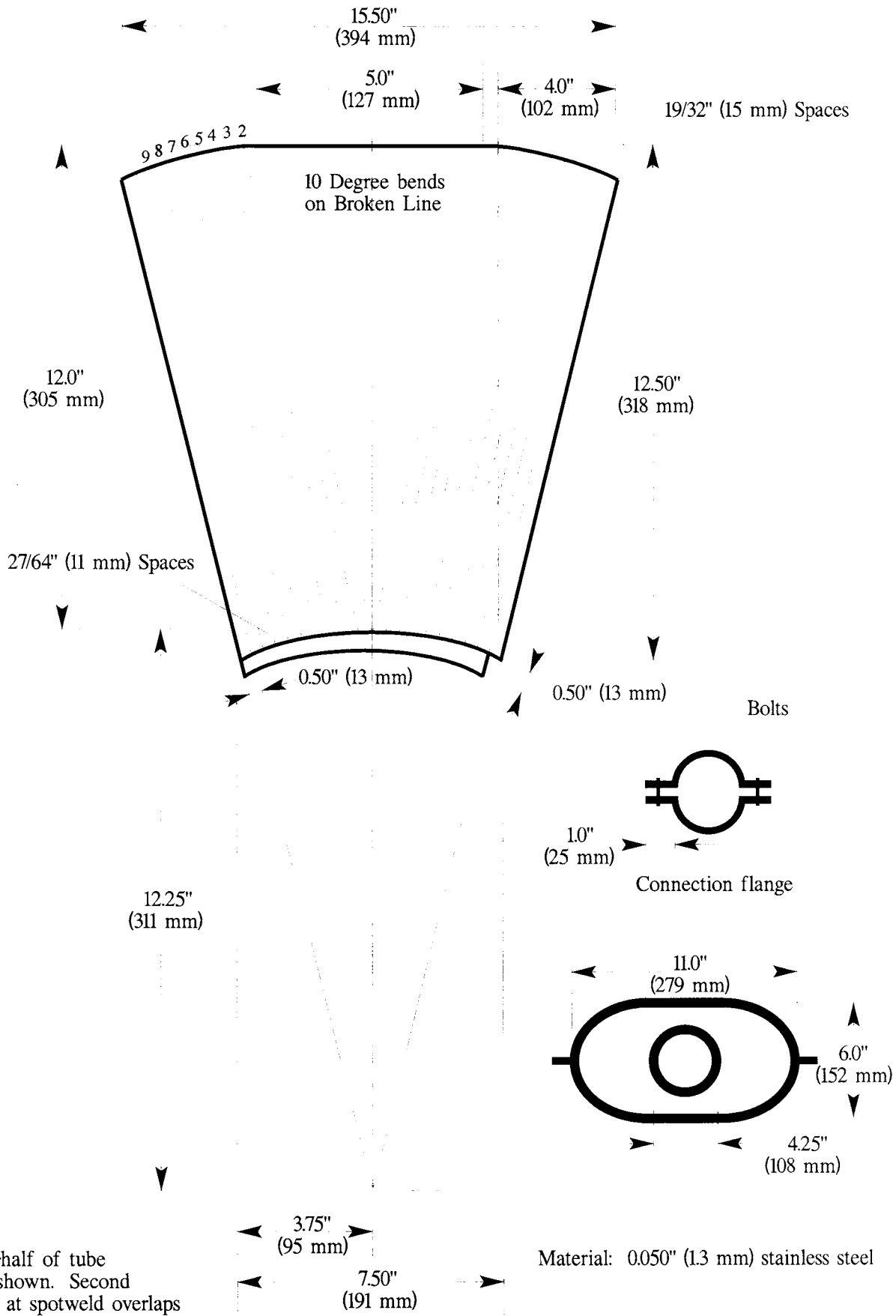
Figure 3 – Burner Draft Tube Extension Cone Diagram
